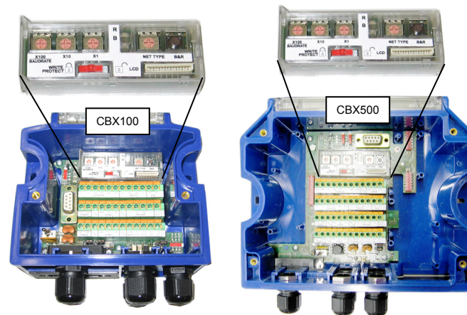
Figure 2 – BM100 Mounting
